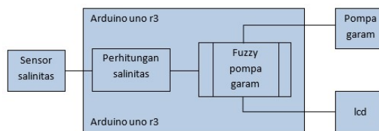
Gambar 1 Blok Diagram
