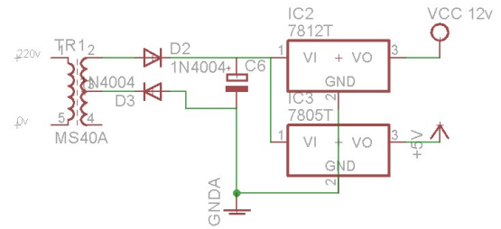
Gambar 4 Rangkaian Power Supply 12 V
