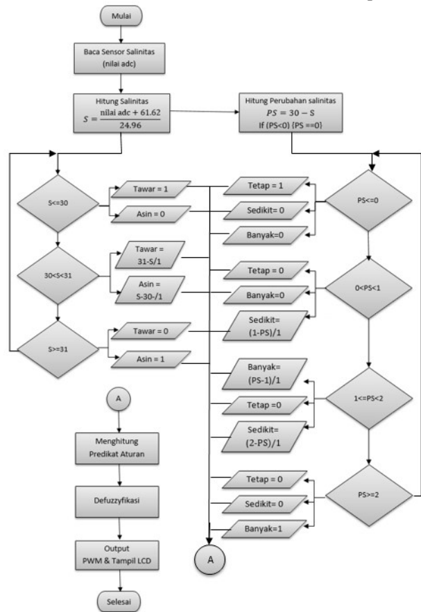
Gambar 8 Flowchart Program
